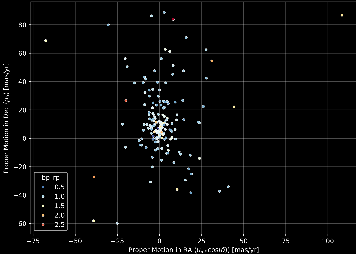
APOGEE DR17 Field: [288-28-O_TESS] Proper Motion Diagram (n= 170)
