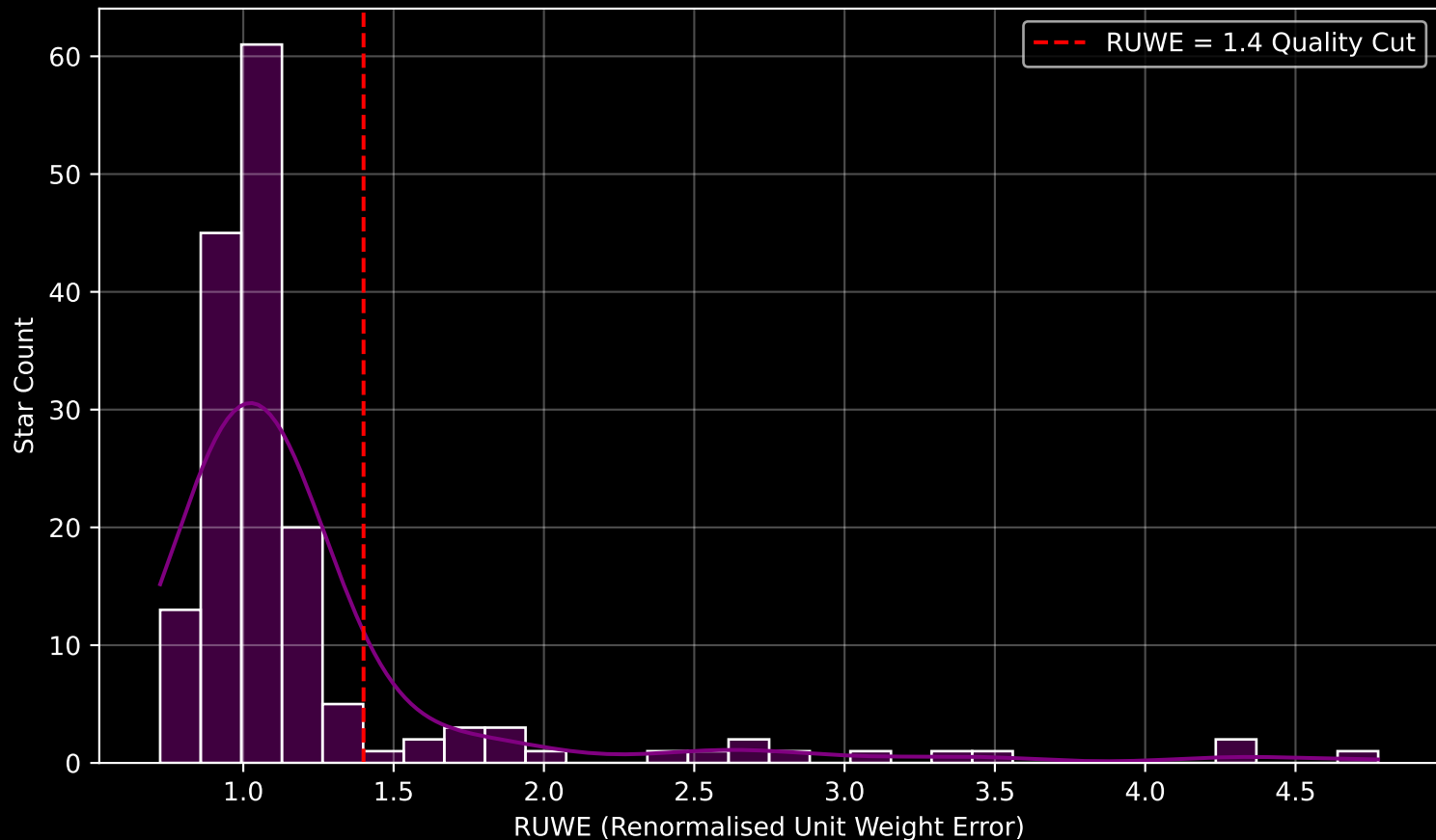
GAPOGEE DR17 Field [288-28-O_TESS] RUWE Distribution (n= 165)
