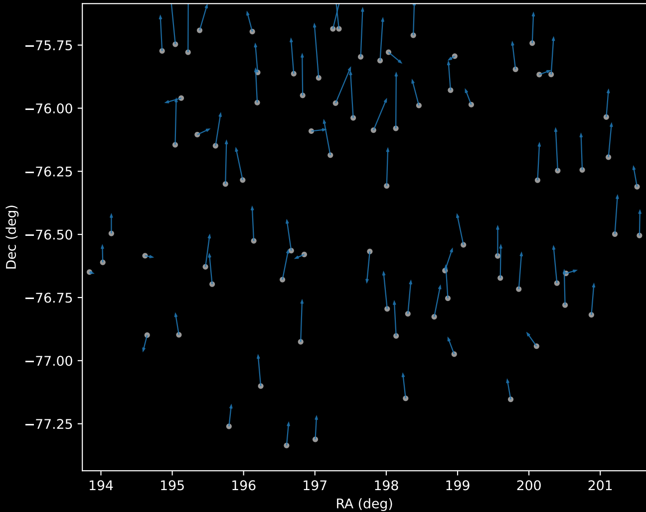
APOGEE DR17 Cluster 0 Proper Motion Vectors (n=81)
