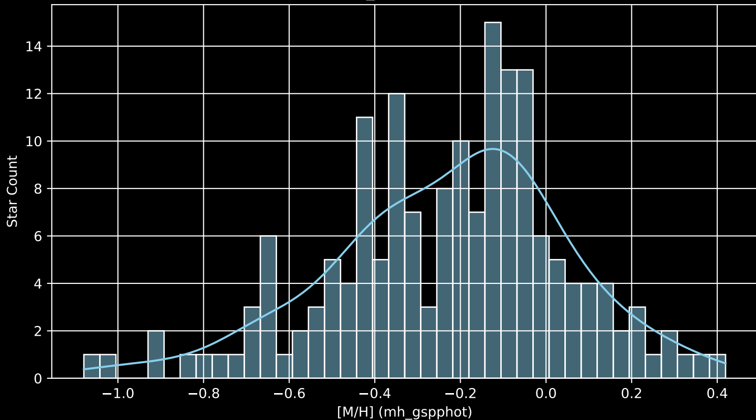
APOGEE DR17 Field: [288-28-O_TESS [M/H] (mh_gspphot) (n= 170)
