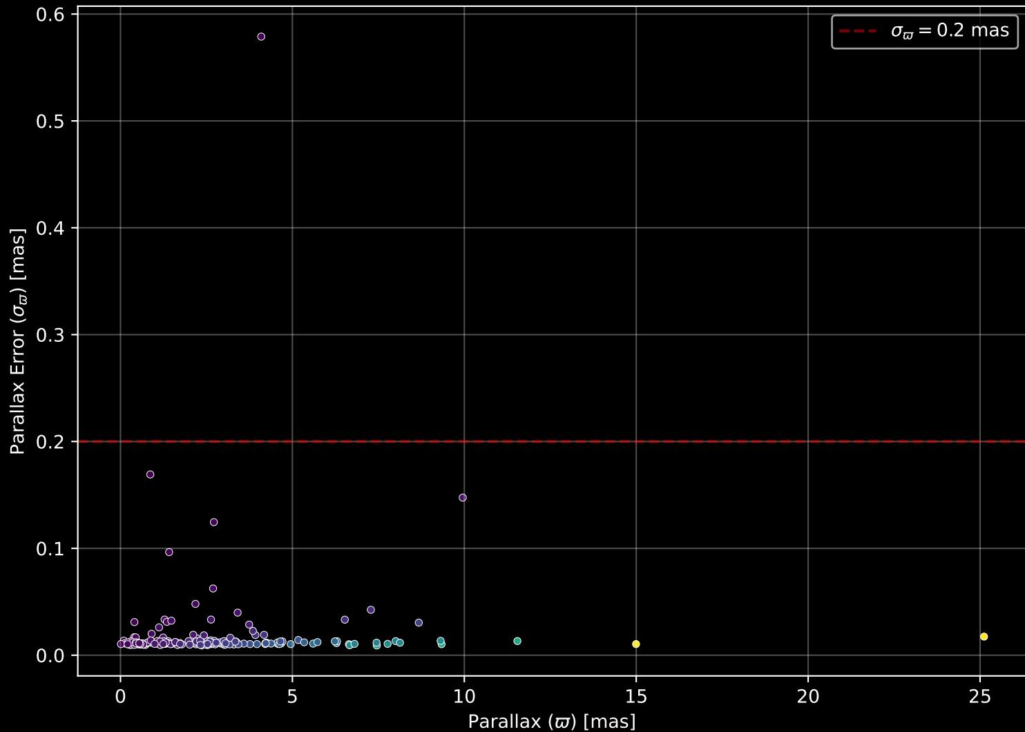
APOGEE DR17 Field: [288-28-O_TESS] Parallax Quality (n= 170)
