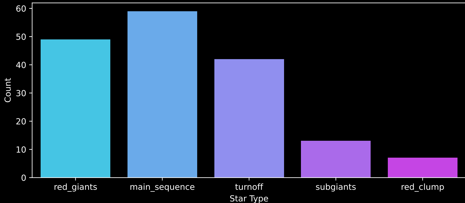
APOGEE DR17 Field: [288-28-O_TESS] Count plot of Star Type
